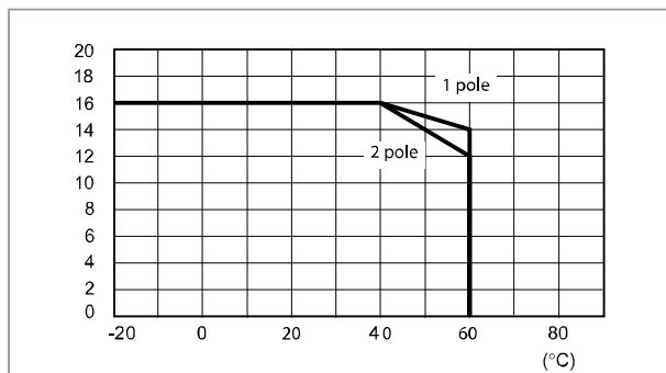
L 12 - Rated current v ambient temperature
