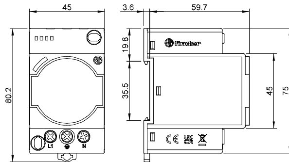
Type 7U.02 Box clamp
